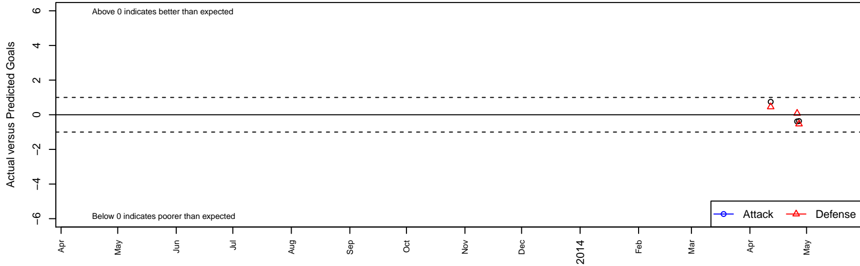
BYSC Corona United B99 Dots are actual minus expected GF (blue circles) and GA (red triangles). Blue line is smoothed change in attack strength. Red is smoothed change in defense strength.
